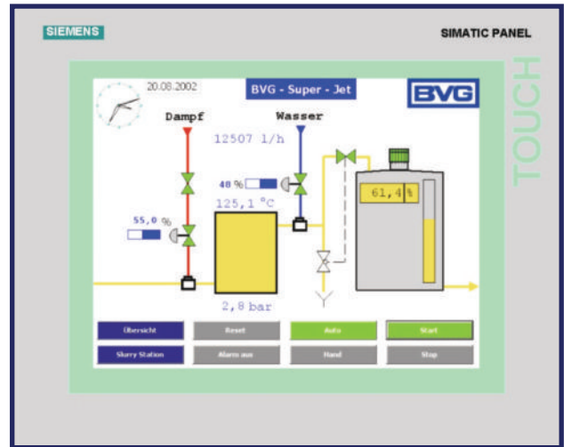
Monitoring Jet-Cooker
